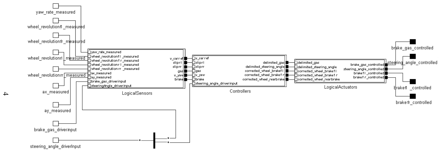
Figure 1: Architecture of the vehicle stability control system
