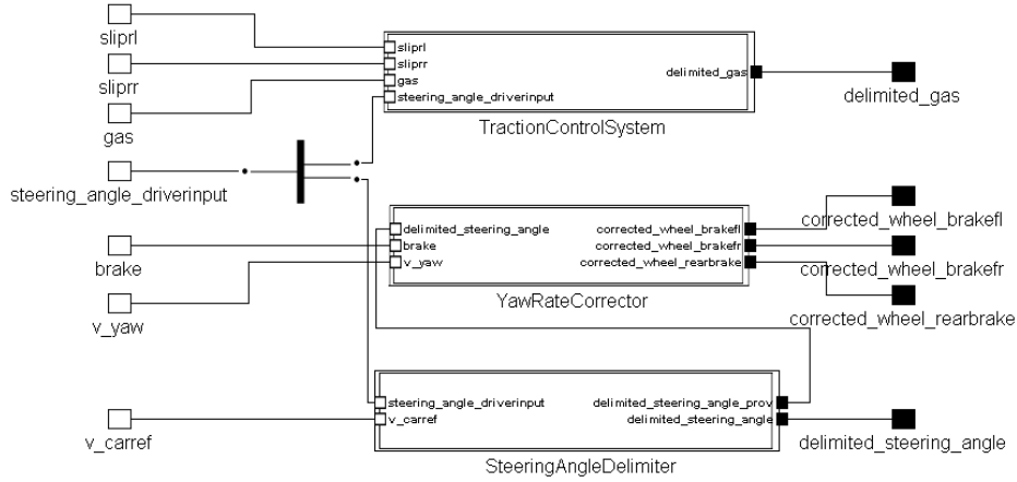
Figure 2: Internal structure of the controller component
