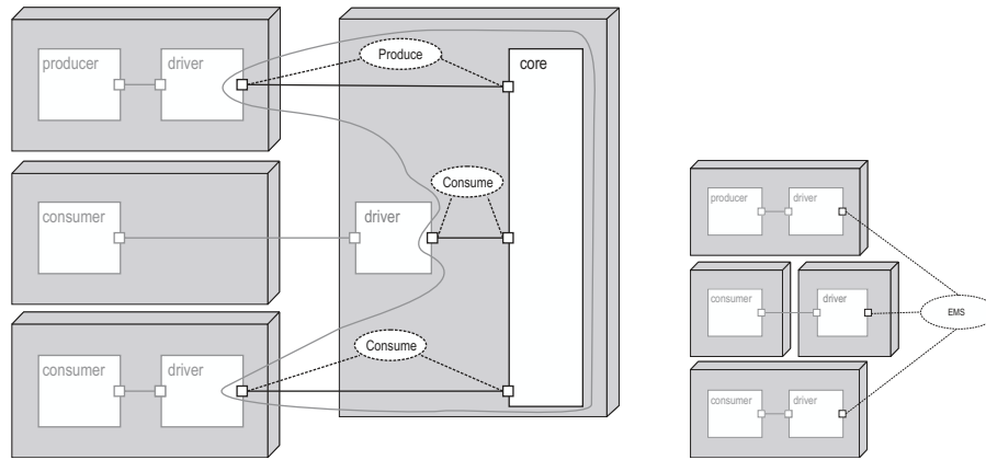
Figure 1: Architecture for the software of the energy management system (cf. [RSS05, Gie08])
